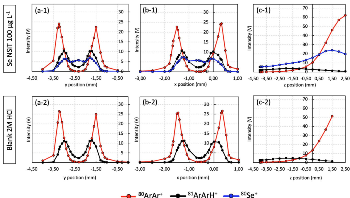
Fig. 1 Radial ( x , y ) and axial ( z ) spatial profiling of ^{80}\text{ArAr}^+ , ^{81}\text{ArArH}^+ and ^{80}\text{Se}^+ with a fixed carrier gas flow rate of 1.2 \text{ L min}^{-1} . For radial profiling, the z position was fixed at -4.0 \text{ mm} .
