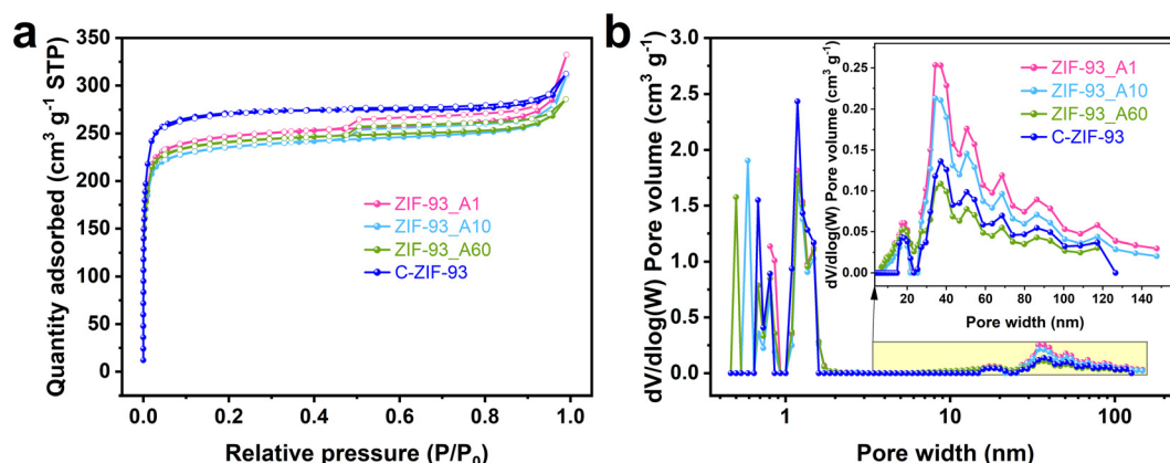
Fig. 4 (a) N 2 adsorption–desorption isotherms and (b) pore size distributions of ZIF-93_At and C-ZIF-93 samples.
