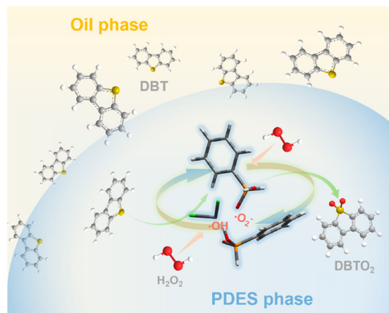
Scheme 1 ECODS mechanism using the bifunctional PDES \text{ZnCl}_2/2\text{PIA} .
