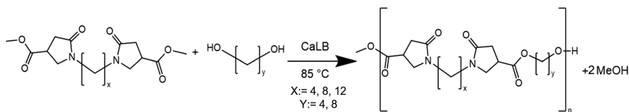
Fig. 3 Reaction scheme of BPdm-based polycondensation. The reaction between BPdm structures spacers with x = [4, 8, 12] and a potentially bio-based diol with y = [4, 8] in a solventless enzymatically catalyzed reaction formed the BPdm-based oligomers. After 6 h at ambient pressure a further 18 h of reaction time at reduced pressure were applied.
