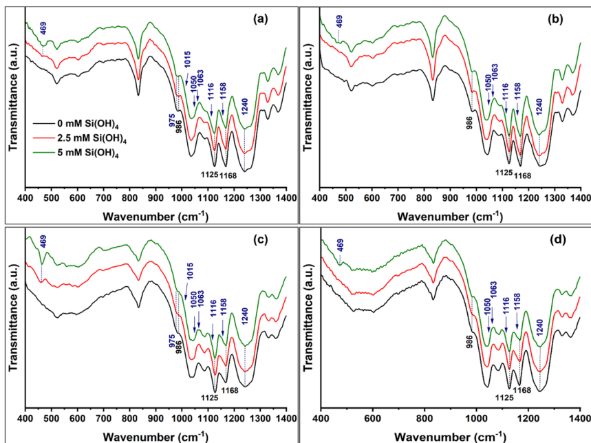
Fig. 7 FTIR transmission spectra of lignin and lignin+Si precipitants. Lignins extracted from biomass of (a) WT, (b) lsi1 , (c) bmr6 and (d) bmr6 × lsi1 plants (black lines) were reacted with silicic acid at 2.5 mM (red) and 5 mM (green) to form lignin+Si precipitates. Peaks and shoulder peaks of Si–O–Si and Si–O–C vibration modes are marked in blue text. Lignin major functional groups, marked in black text, overlapped with silica related peaks. Traces of Si–O–Si absorption band ( 469\text{ cm}^{-1} ) appear when lignin reacted with 2.5 mM silicic acid only in WT and bmr6 . This band is also stronger in lignins extracted from the biomass of WT and bmr6 as compared to lsi1 and bmr6 × lsi1 at 5 mM silicic acid.
