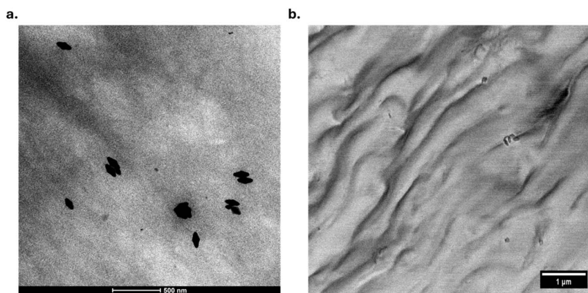
Fig. 4 Microscopy of the three-component hydrogel. (a) TEM image showing the fiber structure of the hydrogel in the background and the darker UCNPs embedded within the gel. (b) SEM image providing a clearer visualization of the hydrogel structure, with the fiber arrangement being more distinct and some UCNPs visible at the surface of the hydrogel.
