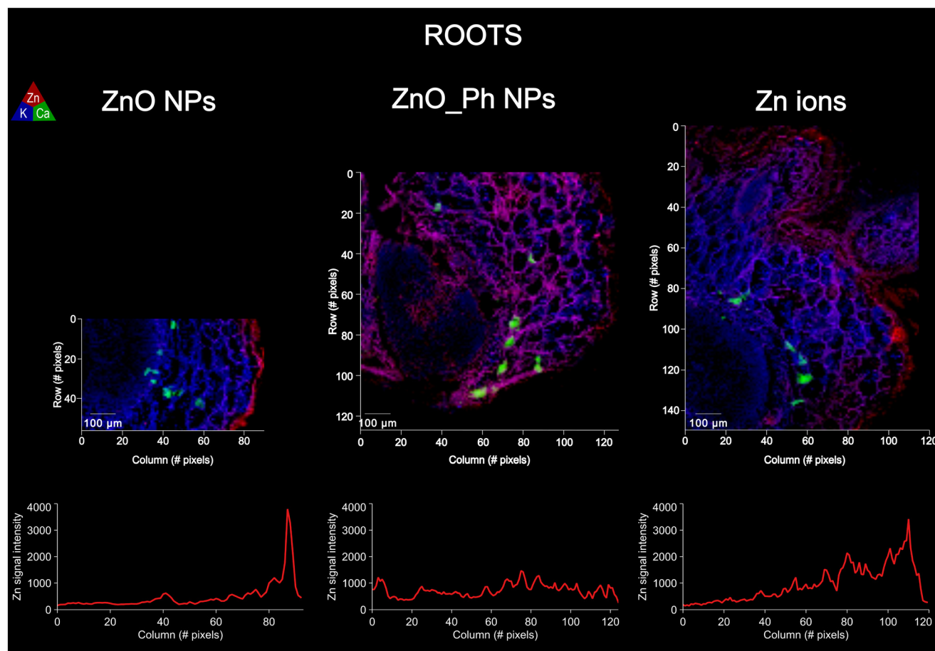
Fig. 2 Elemental \mu -XRF maps on roots of pepper plants exposed to ZnO NPs, ZnO_Ph NPs and Zn ions: one week after exposure. The K\alpha fluorescence of Zn is represented in red, K in blue and Ca in green. Bellow each \mu -XRF map is the average fluorescence intensity measured for Zn along a selected root cross-section. The averaging of Zn K\alpha fluorescence intensity was performed by averaging 3 profiles per \mu -XRF map (Fig. S3†).
