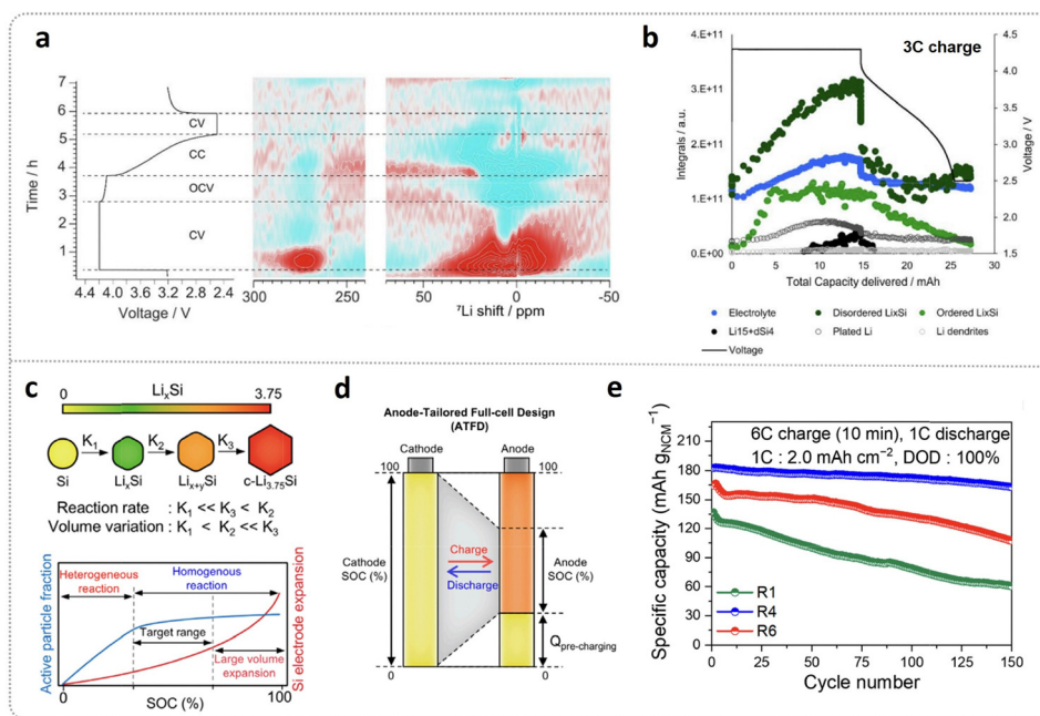
Fig. 5 Achieving fast-charging of full cell with micro-sized Si-C anodes. (a) Contour plots of the time derivative (dOp) of the operando ^7\text{Li} NMR intensities. (b) Capacity evolution of the integrals of the deconvoluted peaks corresponding to the responses from the ^7\text{Li} nuclei in various cell environments in the spectra from the operando ^7\text{Li} NMR experiment during the cycle with 3C charge, 110 with permission from American Chemical Society, 2023. (c) Reaction rate and volume variation during different lithiation stage of \mu\text{-Si} and trends of active particle fraction and electrode expansion as a function of SOC. ATFD design (d) to achieve the high stability of \mu\text{-Si} -based full cell under ultra fast charge (6C) and (e) corresponding cycling performance, 111 with permission from National Academy of Sciences, 2025.
