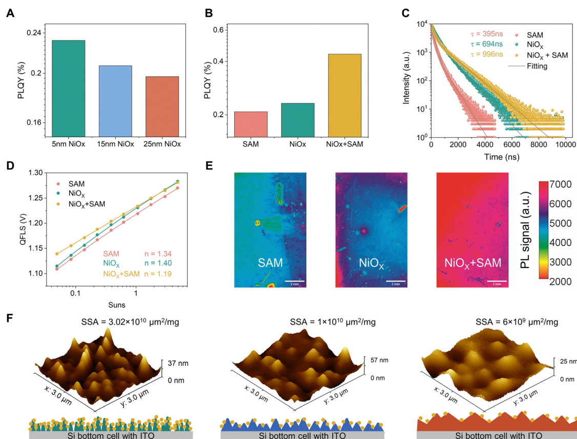
Fig. 3 (A) PLQY measurements performed on half stack samples (Si/ITO/NiO x /2PACz/Perovskite) with different thicknesses of NiO x (5, 15 and 25 nm), showing the highest PLQY at 5 nm, indicating better passivation and reduced non-radiative recombination. (B) PLQY across different HTL configurations (SAM-only, NiO x -only, and NiO x + SAM), demonstrating that the NiO x + SAM combination yields the highest PLQY, suggesting improved interfacial charge carrier management. (C) TRPL measurements reveal prolonged carrier lifetimes for the NiO x + SAM configuration ( \tau = 996 ns) compared to NiO x alone ( \tau = 694 ns) and SAM-only ( \tau = 395 ns), confirming reduced non-radiative recombination and enhanced charge carrier extraction. (D) The Quasi-Fermi Level Splitting (QFLS) measurements show that the NiO x + SAM configuration achieves the lowest ideality factor ( n = 1.19 ), indicative of improved charge transport and suppressed recombination compared to NiO x -only ( n = 1.40 ) and SAM-only ( n = 1.34 ). (E) PL intensity maps performed on half stack samples with different HTLs: Si/ITO/2PACz/Perovskite, Si/ITO/NiO x /Perovskite, Si/ITO/NiO x /2PACz/Perovskite, demonstrating improved film homogeneity. White scale bar: 2 mm. (F) 3D atomic force microscopy (AFM) images of Si bottom solar cells with NiO x layer of different thicknesses (5, 15, 25 nm) and corresponding schematic diagrams of the morphology. The yellow dots indicate SAM molecules anchored onto the NiO x layer. Surface morphology analysis shows that NiO x + SAM forms a discontinuous micro-island structure on the recombination junction, increasing the specific surface area (SSA) significantly ( 3.02 \times 10^{10} \mu\text{m}^2 \text{mg}^{-1} ) compared to NiO x -only ( 1 \times 10^{10} \mu\text{m}^2 \text{mg}^{-1} ) and SAM-only ( 6 \times 10^9 \mu\text{m}^2 \text{mg}^{-1} ). This enhanced SSA promotes better adhesion of SAM molecules, which could improve perovskite nucleation and growth.
