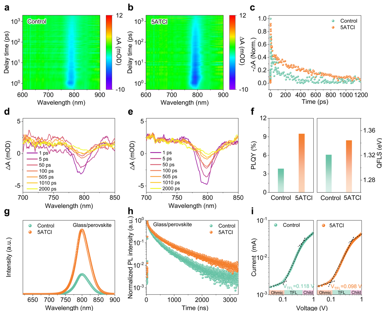
Fig. 3 Properties of perovskite films. The pseudo-color TA plots of the (a) control and (b) 5ATCI-modified perovskite films. (c) The normalized kinetic traces for photo-bleaching probed at 798 nm of the control and 5ATCI-modified perovskite films. TA spectra at different delay times of the (d) control and (e) 5ATCI-modified perovskite films under front excitation. (f) PLQY of different perovskite films deposited on the glass substrates. (g) Steady-state PL spectra and (h) TRPL results of the control and 5ATCI-modified perovskite films. (i) SCLC test of the control and 5ATCI-modified perovskite films.
