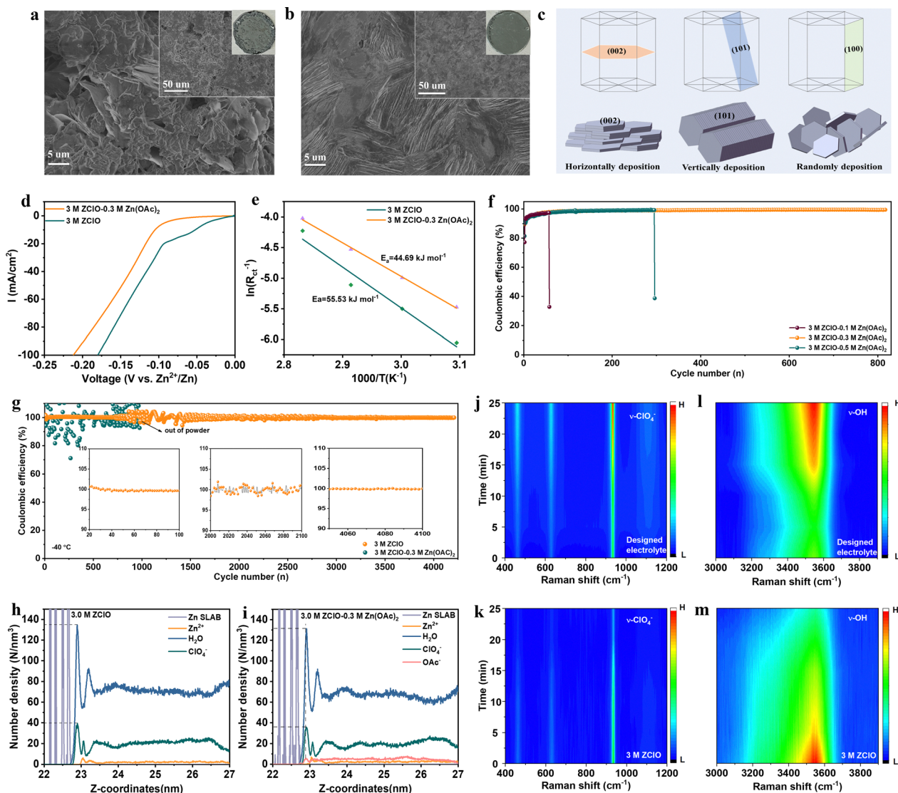
Fig. 4 Interface chemistry and deposition morphology. (a) and (b) SEM images obtained in 3.0 M ZClO (a) and OAc-containing electrolyte (b). (c) Schematic depictions of the Zn plating mechanism. (d) LSV curves of different electrolytes. (e) Activation energy of different electrolytes. (f) Coulombic efficiency of Zn||Cu cells at 1.0 mA cm -2 . (g) Coulombic efficiency at 2.0 mA cm -2 at -40 °C. (h) and (i) Surface electrolyte composition simulated by MD. (j) and (l) In situ Raman results of the electrode/electrolyte interface in 3 M ZClO - 0.3 M Zn(OAc) 2 electrolyte. (k) and (m) In situ Raman results of the electrode/electrolyte interface in 3 M ZClO electrolyte.
