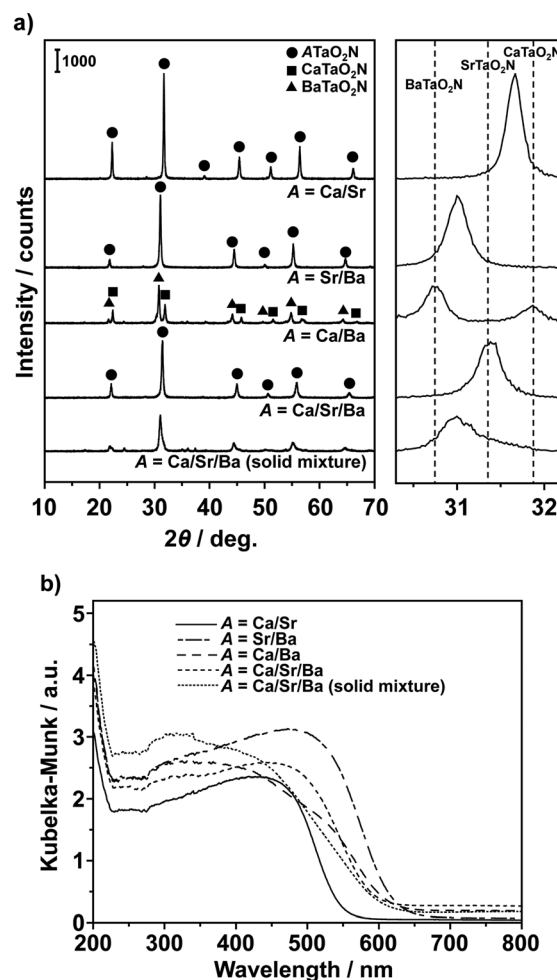
Fig. 1 (a) XRD patterns and (b) Kubelka–Munk-transformed UV-vis DRS of \text{ATa}(\text{O},\text{N})_3 (A = Ca/Sr, Sr/Ba, Ca/Ba, and Ca/Sr/Ba) prepared using PC-derived precursors; data for \text{ATaO}_2\text{N} (A = Ca/Sr/Ba) prepared using a solid powder mixture of \text{ACO}_3 was also shown for comparison. Enlargements of the main reflections at approximately 31^\circ are displayed on the right of panel (a); dashed lines indicate the peak positions of \text{CaTaO}_2\text{N} , \text{SrTaO}_2\text{N} , and \text{BaTaO}_2\text{N} . 46
