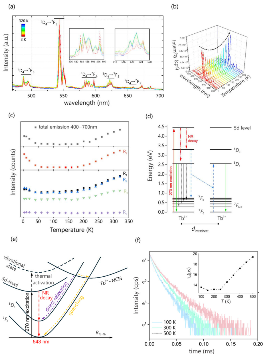
Fig. 3 (a) Emission spectra of Tb 2 O 2 NCN under \lambda_{\text{exc}} = 270 nm in the temperature range between 3 and 320 K, resulting in the transitions ^5D_4 \rightarrow ^7F_J . (b) Temperature-dependent emission spectra showing the anti-thermal quenching effect for the main emission at 543 nm. (c) Temperature-dependence of integrated intensities for the total emission and ^5D_4 \rightarrow ^7F_J transitions, R 1 ( J = 6 ), R 2 ( J = 5 ), R 3 ( J = 4 ), R 4 ( J = 3 ) and R 5 ( J = 2 ). (d) Schematic energy diagram of the cross-relaxation process between ^5D_3 \rightarrow ^7F_0 and ^7F_6 \rightarrow ^5D_4 . (e) Suggested configurational coordinate diagram for the anti-thermal quenching process in Tb 2 O 2 NCN. (f) Decay curves for the transition ^5D_4 \rightarrow ^7F_5 at 100, 300, and 500 K. Inset: temperature-dependence of the experimental radiative lifetime ( \tau_0 ). For the excitation spectrum of Tb 2 O 2 NCN, please see ref. 58.
