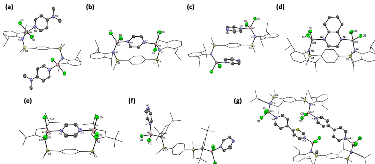
Fig. 2 ORTEP diagram showing the molecular structures of (a) 1-(DMAP) 2 , (b) 1-κ 2 -pyz, (c) 1-(pyz) 2 , (d) 1-κ 2 -qul, (e) 2-κ 2 -pyz, (f) 2-(pyz) 2 , and (g) 1,2-μ-(bipy) 2 (thermal ellipsoids drawn at the 50% probability level for Al, C, Si, N, and O; capped sticks representation for the ligand skeleton; H atoms have been omitted for clarity).
