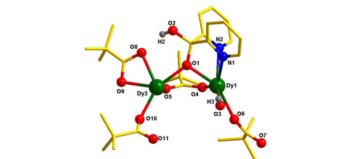
Fig. 1 The asymmetric unit of complex 4. All hydrogen atoms have been omitted for clarity.
