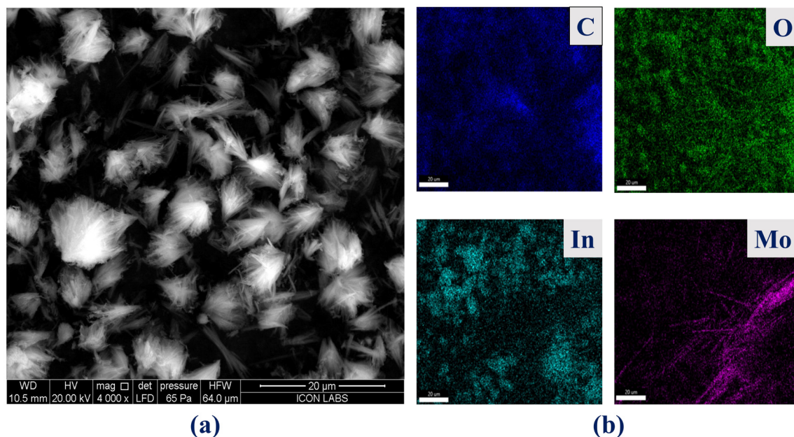
Fig. 8 (a) High-resolution SEM image of Mo 8 O 26 @MIL-117 after four catalytic cycles for oxidative C–N bond formation, highlighting the morphological integrity and surface characteristics. (b) EDX elemental mapping of Mo 8 O 26 @MIL-117 after four catalytic cycles for oxidative C–N bond formation, illustrating the spatial distribution and retention of key elements.
