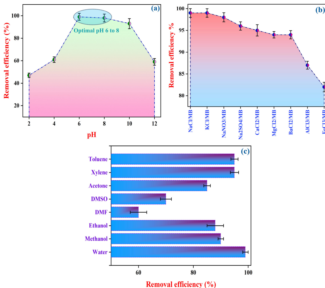
Fig. 10 (a) Influence of pH (2 to 12) on the MB removal efficiency of \text{Mo}_8\text{O}_{26}\text{@MIL-117} . (b) Impact of different salts on MB adsorption performance. (c) Effect of various solvents on the MB removal efficiency of the \text{Mo}_8\text{O}_{26}\text{@MIL-117} composite.
