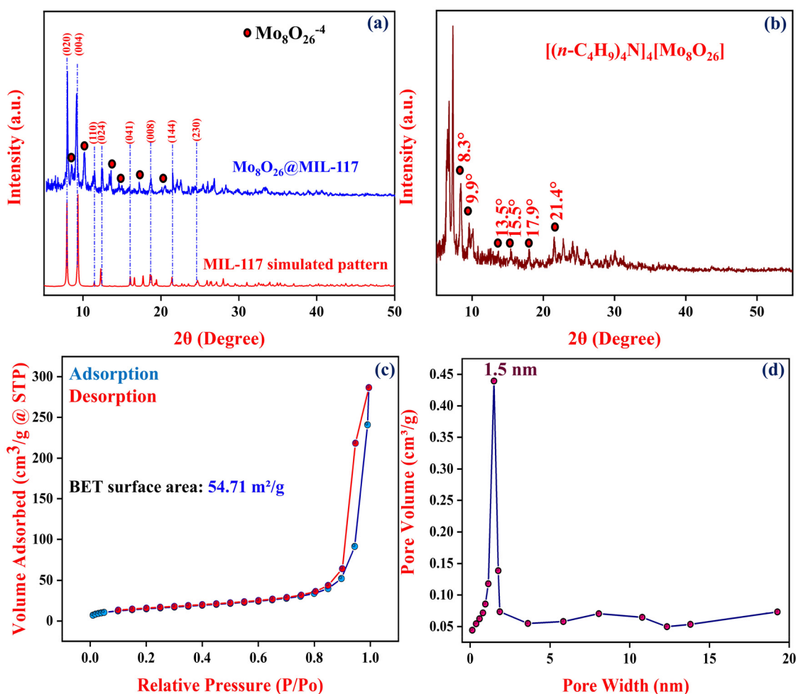
Fig. 4 (a) Comparison of the obtained PXRD patterns of the \text{Mo}_8\text{O}_{26}@\text{MIL-117} composite with the simulated PXRD pattern of MIL-117. (b) PXRD pattern of [(n\text{-C}_4\text{H}_9)_4\text{N}][\text{Mo}_8\text{O}_{26}] . (c) \text{N}_2 adsorption and desorption isotherm of \text{Mo}_8\text{O}_{26}@\text{MIL-117} . (d) BJH pore size distribution diagram of the \text{Mo}_8\text{O}_{26}@\text{MIL-117} composite.
