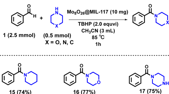
Scheme 2 Oxidative C–N bond formation with benzaldehyde and secondary amines catalysed by \text{Mo}_8\text{O}_{26}@\text{MIL-117} (2 mmol \text{Mo}_8\text{O}_{26}^{4-} loading). Isolated yield in brackets.
