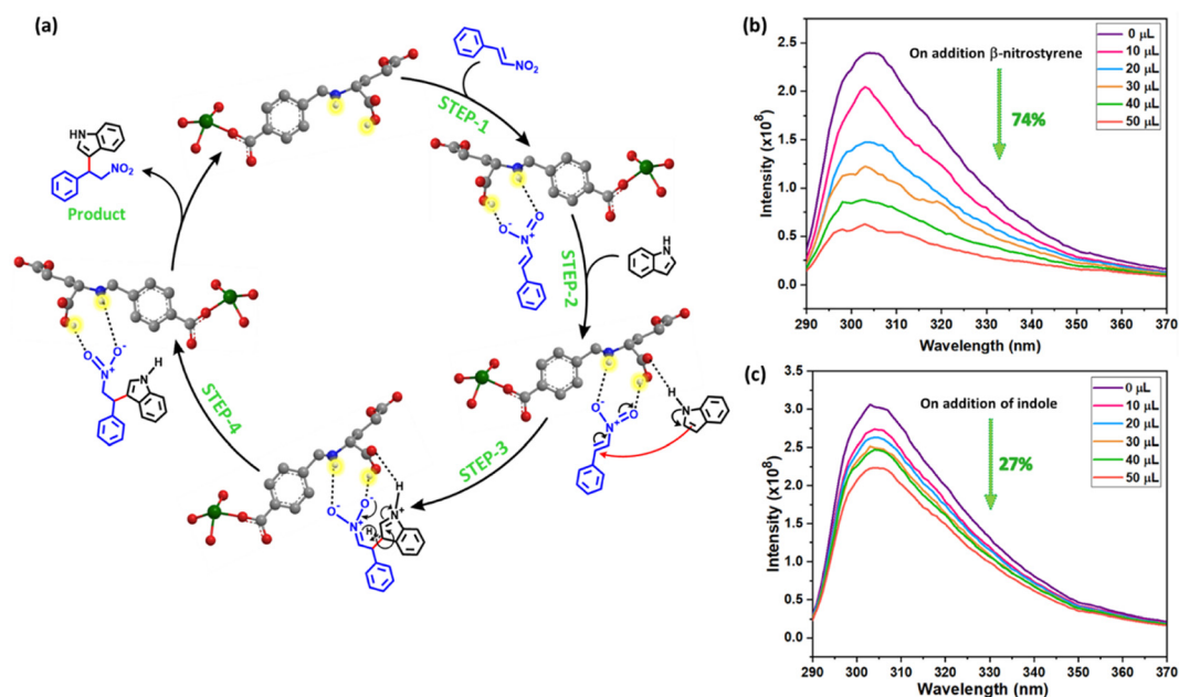
Fig. 8 (a) Propounded catalytic cycle and (b and c) emission spectra ( \lambda_{\text{ex}} = 280 nm) of homogeneous dispersion of Zn-(p-GluBenz) in chloroform on incremental addition of 2 mM solution of \beta -nitrostyrene and indole, respectively.
