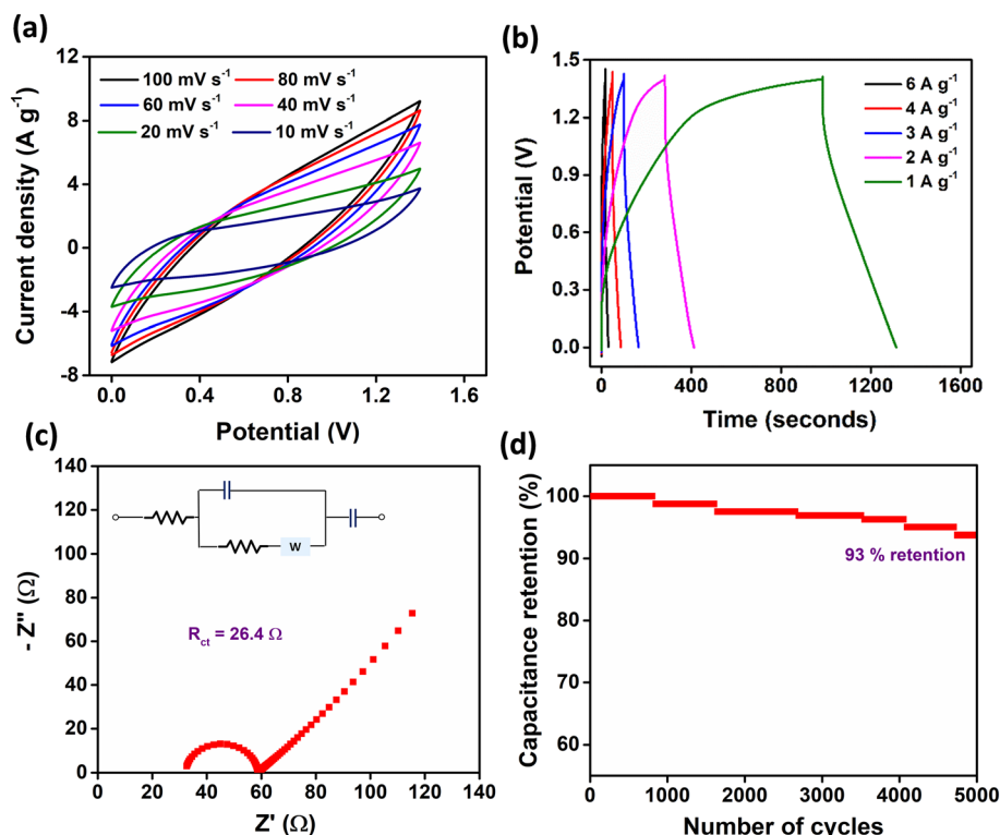
Fig. 6 (a) Cyclic voltammograms of Zn(DAB) at various scan rates, (b) GCD curves at different current densities, (c) Nyquist plot, and (d) cyclic stability of Zn(DAB) at a current density of 6 A g -1 using a two-electrode system.
