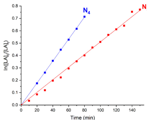
Fig. 3 Kinetic plot for ROP of L-LA promoted by Bn 3 TACN / bTU ( N_3 ) and Bn 4 cyclen / bTU ( N_4 ) depicting a reaction order of unity with respect to the monomer concentration. Pseudo first-order rate constants are: k_{app} = 0.0051 \text{ min}^{-1} ( R^2 = 0.998 ) for Bn 3 TACN and k_{app} = 0.0089 \text{ min}^{-1} for Bn 4 cyclen ( R^2 = 0.997 ).
