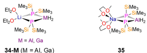
Fig. 9 Heterometallic group 13 \text{P}'' complexes [\text{M}(\text{H})_2(\mu\text{-P}''\text{})_2\text{Li}(\text{Et}_2\text{O})_2] ( 34-M ; M = \text{Al} , Ga), [\text{Al}(\text{H})_2(\mu\text{-P}''\text{})_2\text{Na}(\text{DME})_2] ( 35 ).
