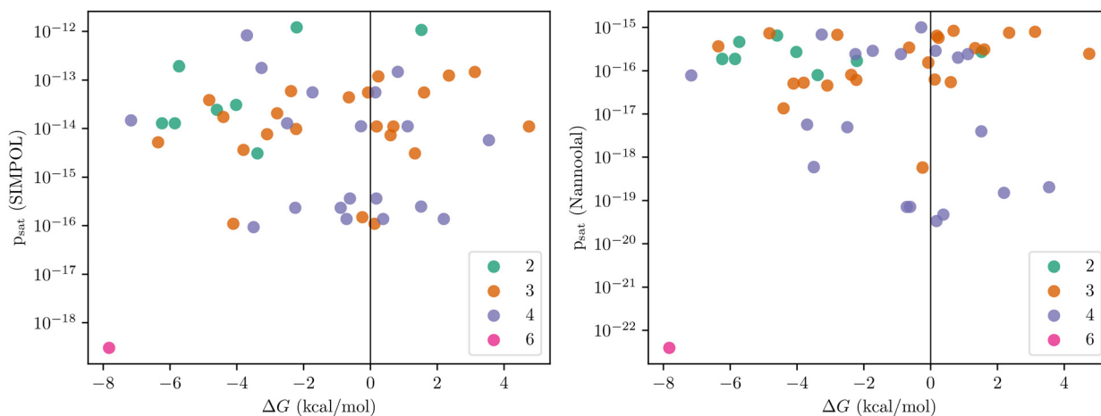
Fig. 3 Binding free energies of 50 homodimers (OOM 2 ) at 298.15 K and 1 atm reference pressure v. SIMPOL and Nannoolal saturation vapour pressures (in atm) of the OOMs. Colors indicate the number hydrogen donors in the corresponding OOM.
