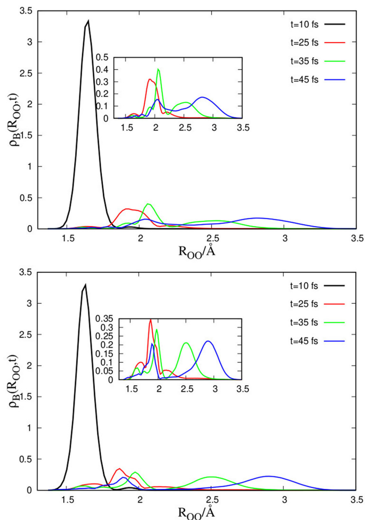
Fig. 17 One-dimensional reduced densities for the B state of the syn - (upper panel) and anti - (lower panel) conformers along R_{OO} are computed using the coupled 3D model. In the inset, we zoom in on the one-dimensional reduced densities for t > 25 fs, where the WP reaches the CAP.
