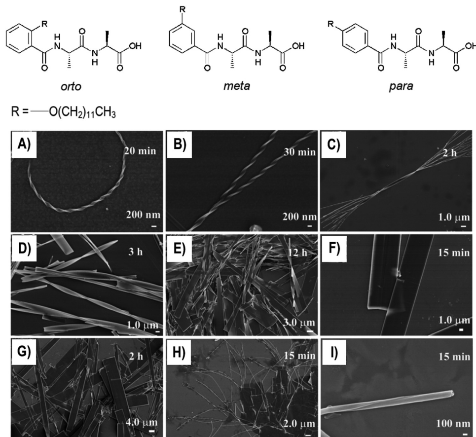
Fig. 24 FE-SEM images of the three dipeptide self-assemblies. All samples were prepared in a CH 3 OH/H 2 O mixed solvent (6/4, v/v) at a concentration of 2.0 g L -1 ; ortho (A)–(E), meta (F) and (G) and para (H) and (I). Reproduced and adapted from ref. 201 with permission from Royal Society of Chemistry, copyright 2021.
