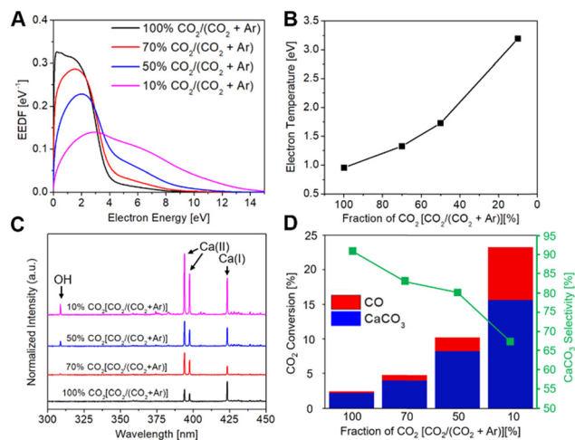
Fig. 5 (A) Simulated electron energy distribution functions and (B) simulated average electron temperatures under varying CO 2 /Ar compositions. (C) Optical emission spectra (300–450 nm) of Ca and \bullet OH spectral lines and (D) CO 2 conversion and CaCO 3 selectivity as a function of CO 2 mole fraction.
