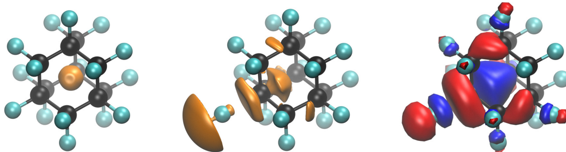
Fig. 6 Left and middle panels: isosurface plots of \Delta ELF for C_{10}F_{16} at the equilibrium geometries of the neutral (left) and anionic (middle) states (isovalue = +0.05 a.u.). Right panel: isosurface plot of the highest occupied molecular orbital of C_{10}F_{16}^- at the equilibrium geometry of the anionic state (isovalue = 0.03 a.u.). The elongated carbon–fluorine bond is shown in the bottom left corner, which is computed at the \omega B97M-V/aug-cc-pVTZ+7s7p level of theory.
