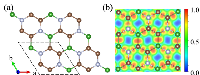
Fig. 1 (a) Top view of the crystal structure of the \text{BC}_2\text{N} monolayer. The unit cell is marked with dotted lines. Green, brown, and grey balls represent boron, carbon, and nitrogen atoms, respectively. (b) Top view of the ELF map.
