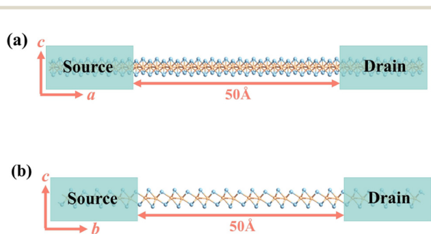
Fig. 3 Schematic diagrams of the two-probe system for computing the electric transport of monolayer O1 variant of ZrCl 2 in (a) the a direction and (b) the b direction. The channel length is 50 Å.
