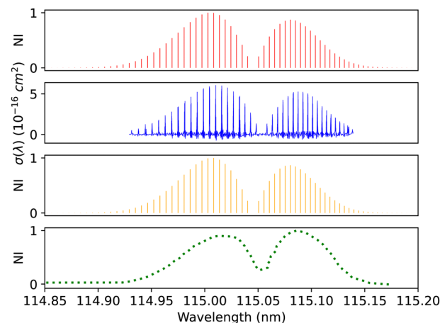
Fig. 12 B^1\Sigma^+-X^1\Sigma^+ (0–0) spectrum: top panel, synthetic band calculated at Eidelsberg et al. 41 experimental conditions. Second panel, calibration (0–0) band due to Eidelsberg et al. 41 Third panel, synthetic band calculated at Federman et al. 106 experimental conditions. Bottom panel, (0–0) band due to Federman et al. 106 NI denotes normalized intensity.
