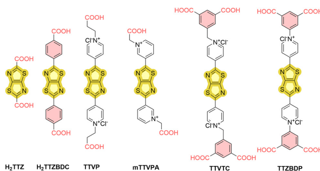
Fig. 3 The TTZ-based multicarboxylic acid ligands for TTZ-based MOFs.
