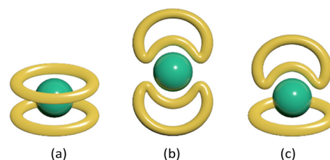
Scheme 1 Sandwich-type macrocyclic complexes with different coordination modes: (a) type A ( face-to-face ), (b) type B ( edge-to-edge ) and (c) type C ( edge-to-face ).
