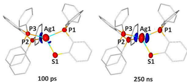
Fig. 2 Photodifference ( F^{\text{ON}} - F^{\text{OFF}} ) maps derived from the Laue experiment indicating electron-density changes 100 ps and 250 ns after excitation plotted on the AgPPPS ground-state geometry. Isosurfaces represent regions with electron density difference of at least \pm 0.35 \text{ e } \text{\AA}^{-3} (left) or \pm 0.55 \text{ e } \text{\AA}^{-3} (right) (blue – positive, red – negative).
