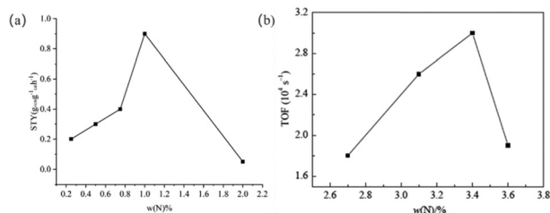
Fig. 9 (a) Space time yield of VCM of xNPCs with various ratios of melamine and PVC ( x = 0.25, 0.50, 0.75, 1.00, 2.00 ). The reaction conditions were 220^\circ\text{C} , \text{GHSV of C}_2\text{H}_2 = 60 \text{ h}^{-1} , \text{HCl/C}_2\text{H}_2 volume ratio = 1.2; 62 reproduced from ref. 62 with permission from American Chemical Society, Copyright 2022. (b) The relationship between nitrogen content and TOF of N-OMC-Ox. 74 Reproduced from ref. 74 with permission from Elsevier, Copyright 2016.
