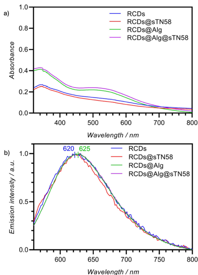
Fig. 3 (a) Absorbance and (b) normalized emission properties of the synthesized systems RCDs, RCDs@TN58, RCDs@Alg and RCDs@Alg@TN58.
