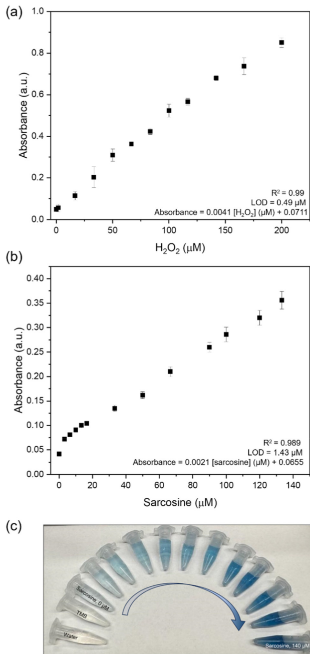
Fig. 4 Detection of H 2 O 2 and sarcosine. (a) Linear calibration curves for varying concentrations of H 2 O 2 with TMB at 1 mM, and (b) varying concentrations of sarcosine using sarcosine oxidase and Cu nanozymes with TMB at 1 mM. Error bars are standard deviations from three replicate measurements. (c) Corresponding images of visible color in the presence of varying concentrations of sarcosine.
