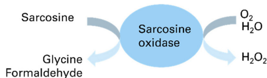
Scheme 1 Reaction scheme for sarcosine catalyzed by sarcosine oxidase enzyme.
