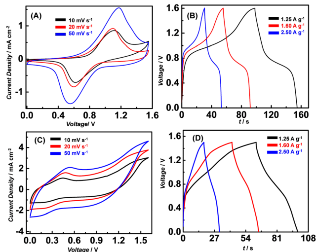
Fig. 5 Electrochemical performances of flavin-based ASCs with a KOH-PEO gel electrolyte: (A) CV plots at different scan rates from 10 to 50 \text{ mV s}^{-1} for cFI //AC ASC, (B) GCD curves at different current densities from 1.25 to 2.5 \text{ A g}^{-1} for cFI //AC ASC, (C) CV plots at different scan rates from 10 to 50 \text{ mV s}^{-1} for FI //AC ASC and (D) GCD curves at different current densities from 1.25 to 2.5 \text{ A g}^{-1} for FI //AC ASC.
