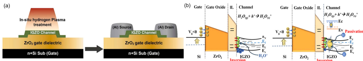
Fig. 8 (a) A cross-sectional schematic of the staggered bottom gate a-IGZO TFTs. (b) Energy band diagrams of a-IGZO TFTs under NBS without and with in situ hydrogen plasma treatment. Reproduced with permission. 112 Copyright 2024, J. H. Wu, Nanotechnology.
