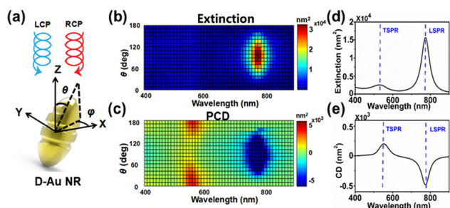
Fig. 2 Influence of orientation of D-Au NR to the light incidence on the PCD response. (a) Schematic of the incident left/right-polarized light along the negative z -axis, and the dc-Au NRs with orientation specified by the polar angle \theta and azimuth angle \varphi . The NRs have a length of 57.5 nm and half-axis of 20 nm along the short axis, respectively, and the chiral feature on the surface has a radius of 15 nm and a helical depth about 10 nm. (b) and (c) Calculated extinction (b) and PCD (c) spectra for \theta = 0^\circ, 10^\circ, 20^\circ, \dots, 180^\circ and \varphi = 0^\circ . The results for fixed \theta do not show significant dependence on the angle \varphi . (d) and (e) Calculated extinction (d) and PCD (e) spectra by integrating the spectra for the angle \theta = 0^\circ, \dots, 180^\circ , \varphi = 0^\circ, \dots, 360^\circ , which resemble the experimental results shown in Fig. 1c and d.
