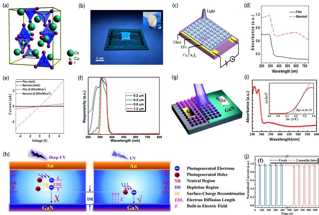
Fig. 6 (a) Crystal structure of Cs 3 Cu 2 I 5 . 83 Copyright 2020, the Royal Society of Chemistry. (b) Digital camera photograph of the DUV photodetector irradiated by 265 nm light. (Inset) DUV photodetector under white light. 77 Copyright 2019, American Chemical Society. (c) Schematic diagram of DUV detection based on nano-hollow Cs 3 Cu 2 I 5 . (d) Absorption curves of the Cs 3 Cu 2 I 5 thin film and nanonet. (e) I – V curves of the Cs 3 Cu 2 I 5 nanonet and film photodetector under 275 nm irradiation with 0.095 mW cm −2 and in the dark. 82 Copyright 2022, by the authors. Licensee MDPI, Basel, Switzerland. (f) Response spectra of the photodetector with different absorber thicknesses. (g) Schematic illustration of the Cs 3 Cu 2 I 5 /GaN heterojunction device. (h) Schematic diagram of the work mechanism. 83 Copyright 2020, the Royal Society of Chemistry. (i) Absorption spectrum and the corresponding optical band gap (inset) of the Cs 3 Cu 2 I 5 thin films deposited at 110 °C. 84 Copyright 2021, Optical Society of America. (j) Stability evaluation of the photodetector after 2 months of storage in open air. 86 Copyright 2021, American Chemical Society.
