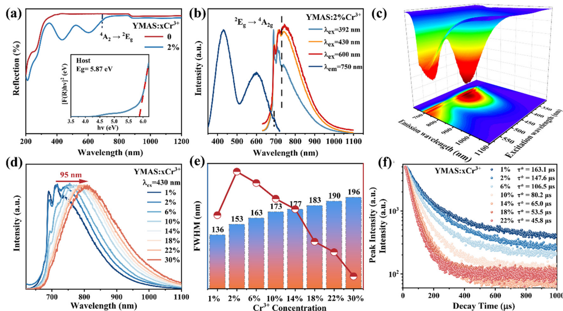
Fig. 2 (a) UV-vis-NIR DR spectra of YMAS:xCr 3+ ( x = 0, 2\% ). The illustration is the optical band gap of the YMAS host. (b) PL and PLE spectra of YMAS:2%Cr 3+ . (c) The PL mapping spectrum of YMAS:2%Cr 3+ . (d) Normalized PL spectra of YMAS:xCr 3+ ( x = 1-30\% ). (e) Luminescence peak intensity and FWHM of YMAS:xCr 3+ ( x = 1-30\% ). (f) Fluorescence decay curves of YMAS:xCr 3+ ( x = 1-22\% ) at the optimal monitoring wavelength (715–810 nm).
