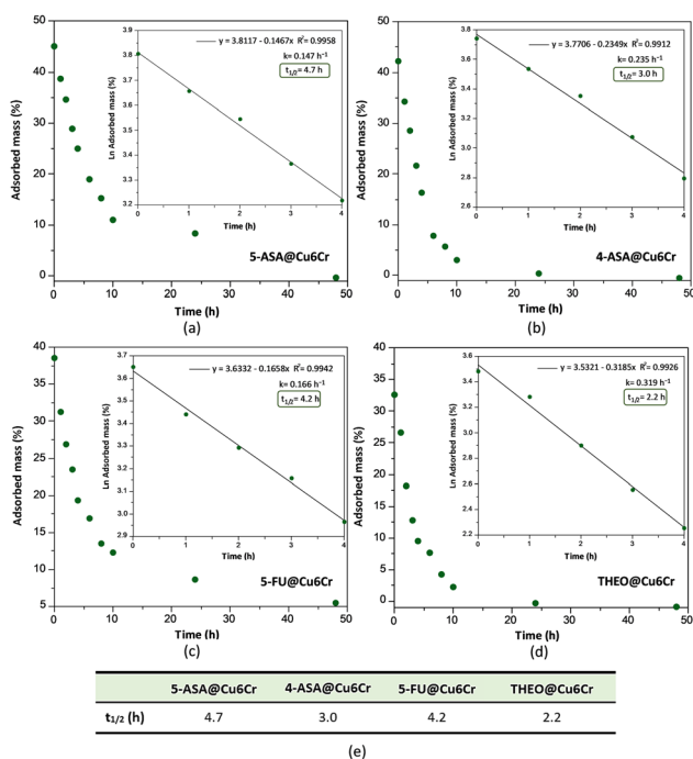
Fig. 3 Kinetic desorption curves in water at 35 °C for (a) 5-ASA@Cu _6 Cr, (b) 4-ASA@Cu _6 Cr, (c) 5-FU@Cu _6 Cr and (d) THEO@Cu _6 Cr. Inset: Fitting to first-order kinetics considering the first 4 h of the desorption process. (e) t_{1/2} values.
