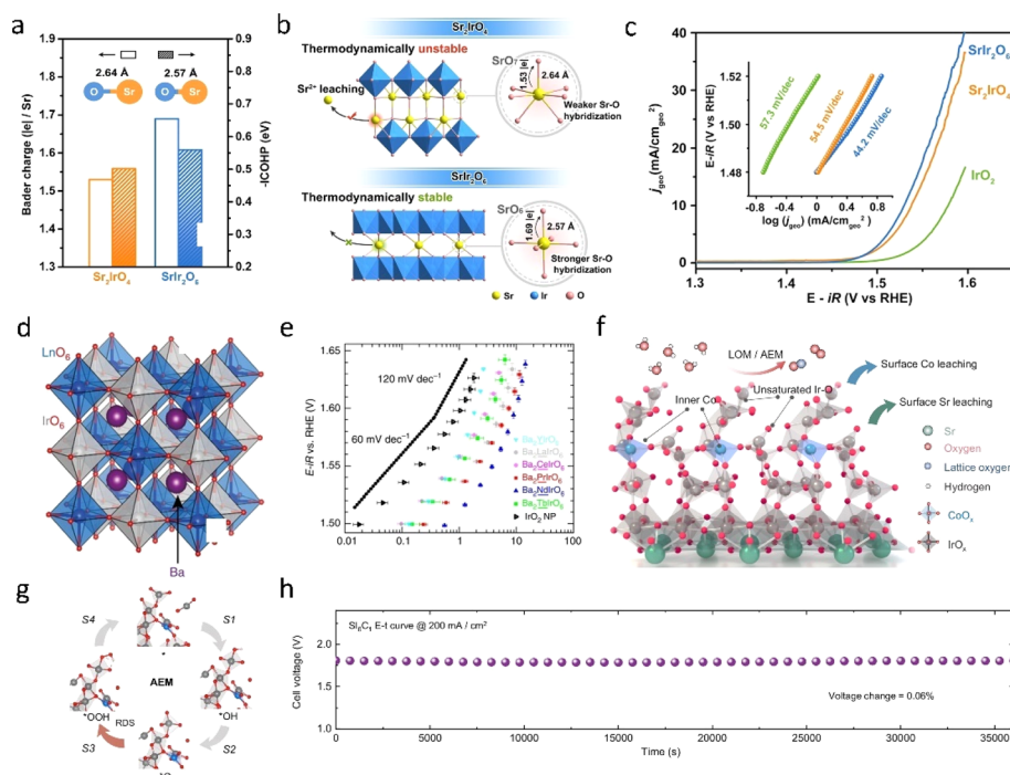
Fig. 6 (a) Sr–O bond length, the integrated –ICOHP values of the Sr–O bond, and the Bader charge analysis of SrIr 2 O 6 and Sr 2 IrO 4 . (b) Schematic showing the key factors controlling the structural stability of SrIr 2 O 6 and Sr 2 IrO 4 . (c) Linear polarization curves for the OER of SrIr 2 O 6 , Sr 2 IrO 4 , and IrO 2 at 1 mV s -1 in a 0.1 M HClO 4 electrolyte, with the corresponding Tafel slopes in the inset. 61 Copyright 2023, American Chemical Society. (d) Crystal structure of a generic Ba 2 MlIrO 6 DP. (e) OER activity in 0.1 M HClO 4 of Ba 2 MlIrO 6 , compared with the benchmark activity of IrO 2 nanoparticles; the dotted lines show Tafel slopes of 60 and 120 mV per decade. 31 Copyright 2016, Springer Nature. (f) OER catalytic mechanism diagram of the Co doped SrIrO 3 catalyst. (g) Adsorbate evolution mechanism (AEM) diagram. (h) OER performance of the samples. 63 Copyright 2024, Springer Nature.
