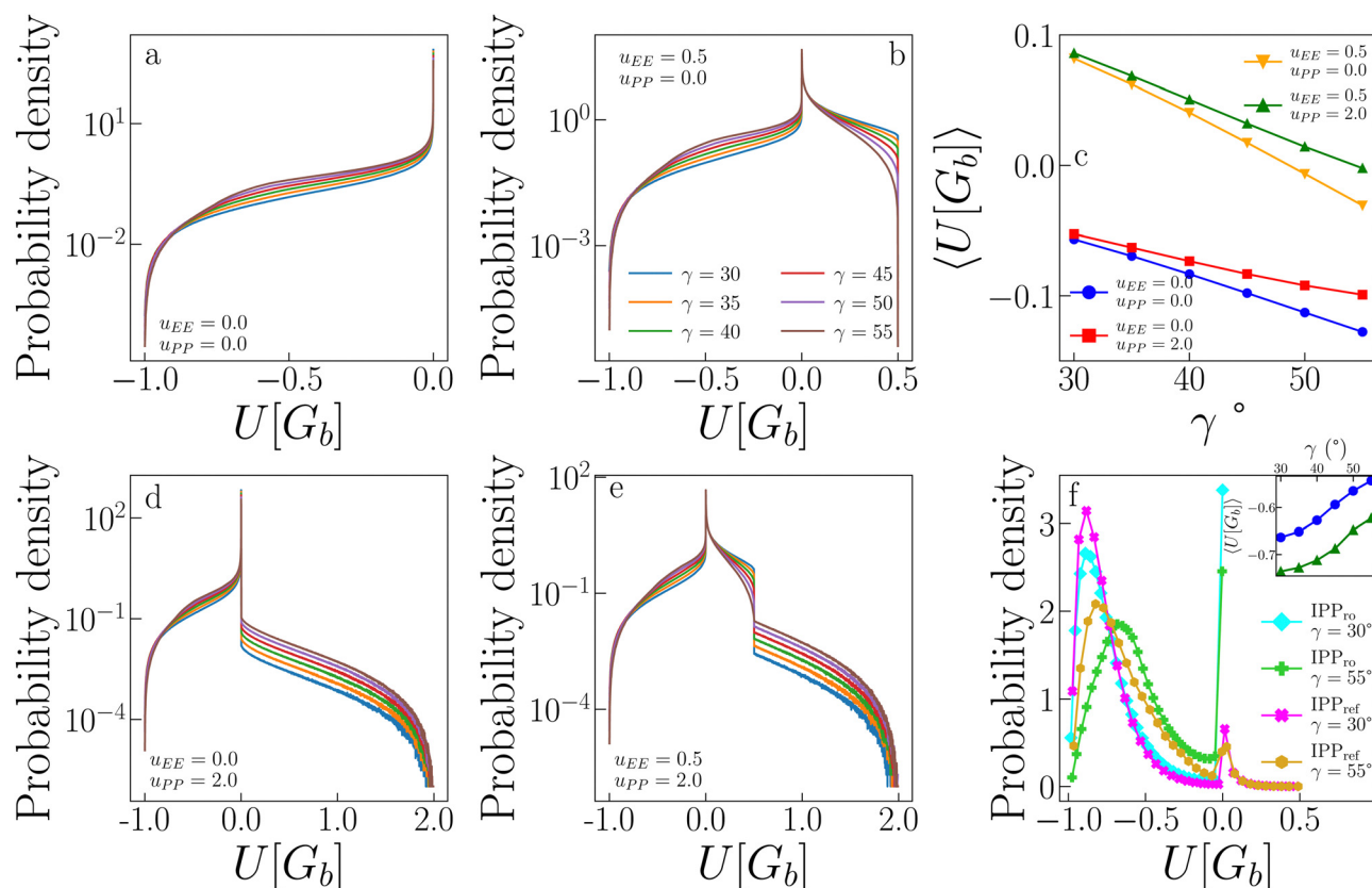
Fig. 7 Impact of patch-patch repulsion on the energy of IPP systems. (a) Distributions of the energy of geometric bonds for randomly generated pair configurations of IPPs with u_{EE} = 0.0 and different values of \gamma . (b) Same as in (a), but for IPPs with u_{EE} = 0.5 and u_{PP} = 0.0 . (d) Same as in (a), but for IPPs with u_{EE} = 0.0 and u_{PP} = 2.0 . (e) Same as in (a), but for IPPs with u_{EE} = 0.5 and u_{PP} = 2.0 . (c) Average of the distributions shown in panels a, b, d and e. (f) Distributions of the energy of geometric bonds for configurations observed in simulations at the critical point for IPP ro and IPP ref systems, i.e., systems with u_{EE} = 0.0 , u_{PP} = 0.0 and u_{EE} = 0.5 , u_{PP} = 2.0 respectively, for \gamma = 30 and \gamma = 55 . Inset: Average of the distributions shown in panel f.
