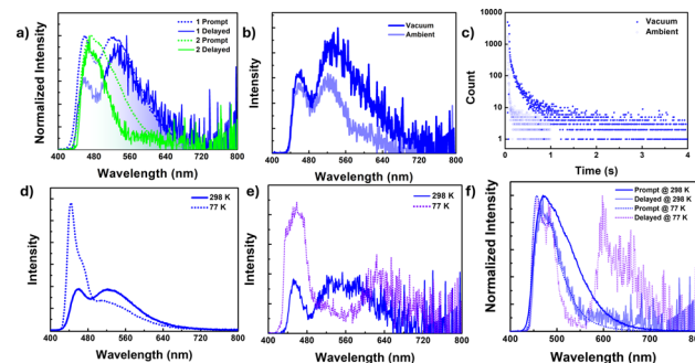
Fig. 3 (a) Prompt and delayed (50 \mu\text{s} delay) PL spectra for 1 and 2 in solid state (as prepared) [ \lambda_{\text{ex}} = 380 nm], (b) time-gated PL spectra (50 \mu\text{s} delay) and (c) delayed fluorescence lifetime decay [ \lambda_{\text{em}} = 520 nm] for 1 (as prepared) [ \lambda_{\text{ex}} = 380 nm] at 298 K under vacuum (absence of oxygen) and ambient conditions (presence of oxygen). (d) Fluorescence spectra and (e) time-gated spectra [50 \mu\text{s} delay] for 1 under a vacuum atmosphere at 298 K and 77 K upon \lambda_{\text{ex}} = 380 nm. (f) Normalized prompt and delayed spectra [50 \mu\text{s} delay] for 2 under a vacuum atmosphere at 298 K and 77 K upon \lambda_{\text{ex}} = 380 nm.
