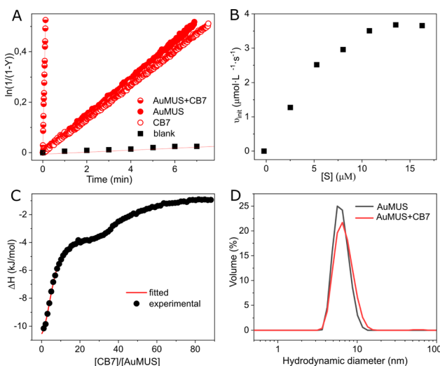
Fig. 3 (A) Kinetic traces for the reaction progress in water (blank), in the presence of the macrocycle (1 equiv.), AuMUS (4 equiv.), and their mixture (1:4), [S] = 0.01 \text{ mM} , water, pH = 6 (adjusted with HCl/NaOH), 298 K; (B) initial rates for CB7–AuMUS (1:4) at varying substrate concentrations; (C) titration of AuMUS with CB7, water, pH = 6 (adjusted with HCl/NaOH), 298 K; (D) the particle size distribution before ( d = 6.41 \pm 0.17 \text{ nm} ) and after the addition of CB7 ( d = 6.86 \pm 0.10 \text{ nm} ).
