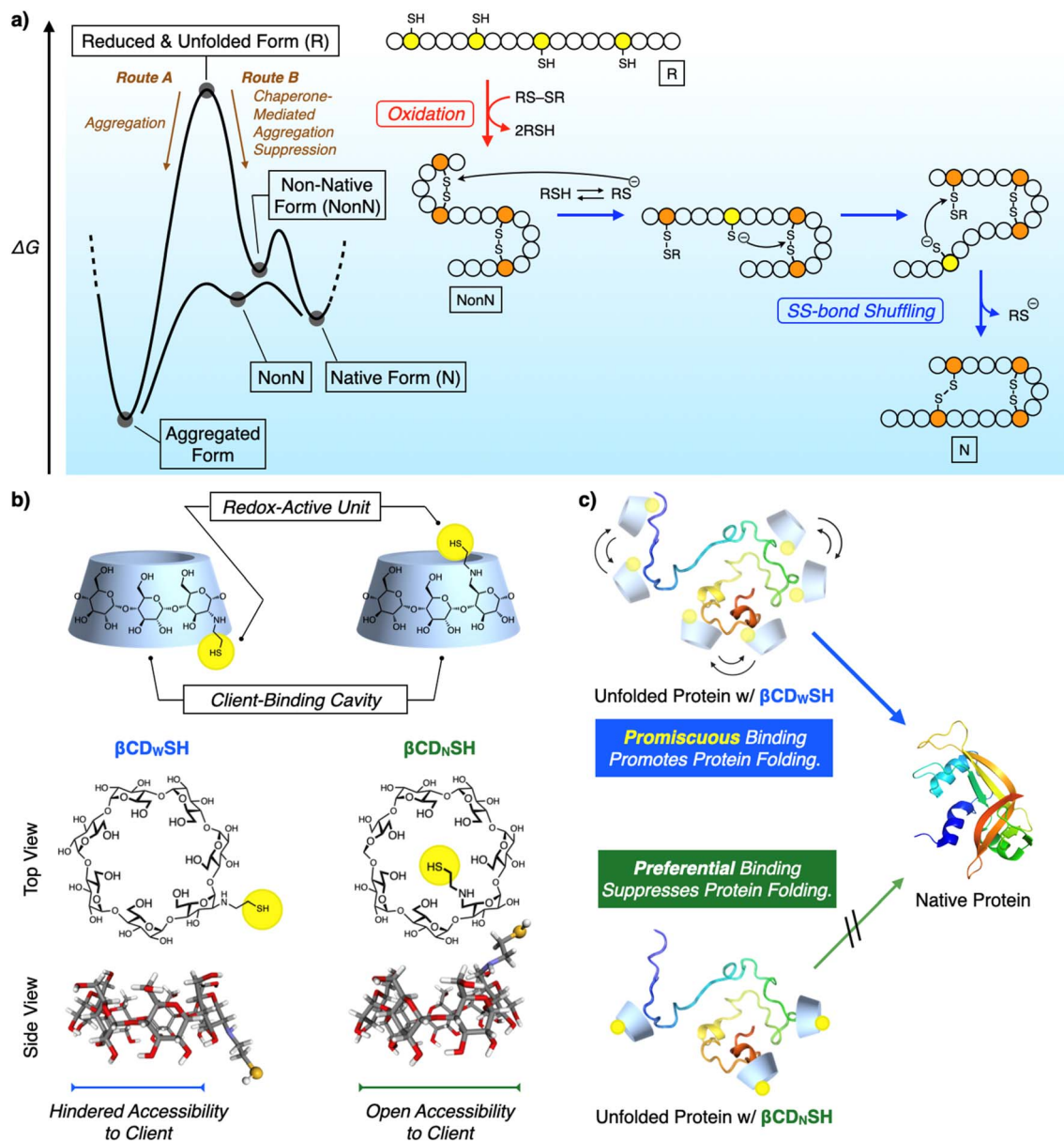
Fig. 1 (a) Schematic illustration of the oxidative folding of a polypeptide chain. Yellow and orange circles represent cysteine residues that are in the thiol/thiolate form and disulfide form, respectively. Open circles represent amino acid residues other than cysteine. Red arrow step: oxidation reaction from a reduced and unfolded form (R) to a non-native form (NonN). Blue arrow steps: disulfide bond isomerization from NonN to N by the nucleophilic attack of thiolates. (b) Molecular structures of \beta\text{CD}_w\text{SH} and \beta\text{CD}_n\text{SH} . Schematic images showing the redox-active units and client-binding cavities, and the molecular models calculated using DFT B3LYP 6-31G*. (c) The concept of (blue) the promiscuous binding property of \beta\text{CD}_w\text{SH} and (green) the preferential binding property of \beta\text{CD}_n\text{SH} with an unfolded protein. The promiscuous binding property of \beta\text{CD}_w\text{SH} is advantageous for promoting protein folding compared to the preferential binding property of \beta\text{CD}_n\text{SH} .
