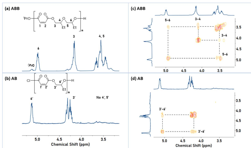
Fig. 1 Comparison of ^1\text{H} and COSY NMR spectra for P1 (ABB) and P1' (AB). Left: Selected regions of the ^1\text{H} NMR spectra (400 MHz, \text{CDCl}_3 referenced at 7.26 ppm), illustrating the methine and methylene resonances for P1 (ABB) (a) and P1' (AB) (b). Right: Magnified ^1\text{H} COSY NMR spectrum of P1 (ABB) (c) and P1' (AB) (d). Full spectra are available in Fig. S1, S3, S80 and S81.†
