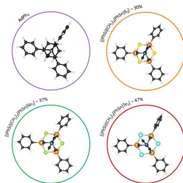
Fig. 27 Atomic structure calculated within DFT in the independent particle approximation for AdPh 4 ( 1016 , top left) and different tetraphenyl clusters with modified cluster cores. The circle color corresponds to the respective line color of the second order optical response shown in Fig. 28. 642,644
