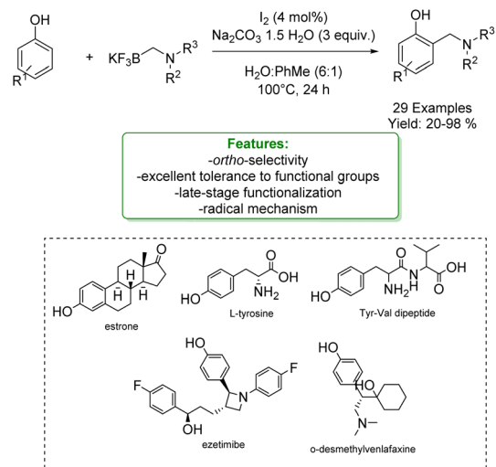
Scheme 38 Iodine-sodium percarbonate catalysed aminomethylation of phenols with trifluoroborate reagents. 125
