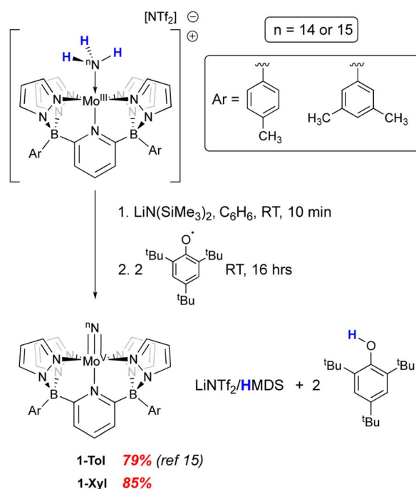
Scheme 2 Synthesis of neutral \text{Mo}(\text{v}) nitrido derivatives 1-Ar ( \text{Ar} = \text{para-tolyl, meta-xylyl} ).
