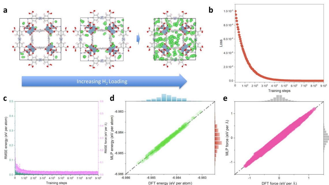
Fig. 2 MLP derivation for \text{H}_2 @Al-soc-MOF-1d. (a) Illustration of the \text{H}_2 @Al-soc-MOF-1d host-guest model systems with different \text{H}_2 loading (from 8 to 134 molecules per unit cell) selected for the generation of the training/validation data points by AIMD simulations. (b) Variation of the loss function over the training loops. (c) Training RMSE of energy and force changes over the training loops. (d and e) Training test with randomly 500 selected configurations from the training datasets (detailed information can be found in the Computational methods section).
